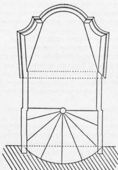
Fig. 4. Plan av predikstolen i Kung Karls kyrka. — Plan of the Pulpit in the Church of Kung Karl.
