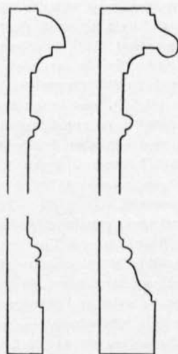
Fig. 5. Profiler till Kung Karls kyrkas predikstol. T.v. tillbyggd del, t.h. ursprunglig del. — Outline drawings of the Pulpit in the Church of Kung Karl; on the left, the added part, and on the right the original portion.
